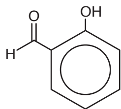
salicylaldehyde ( 197^{\circ}\text{C} )
